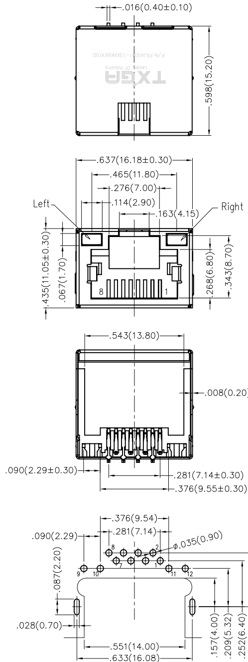
Recommended P.C.Board Layout
